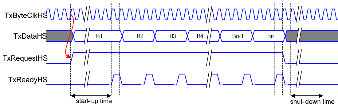
1724 1725 Figure 58 Example High-Speed Transmit from the Slave Side
