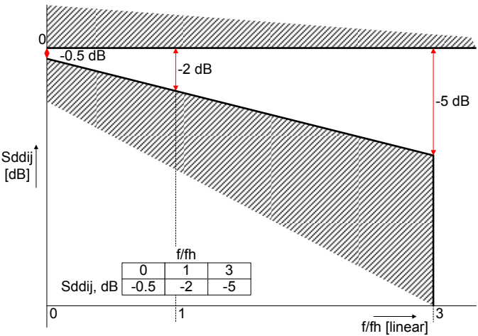
1231 1232 Figure 28 Template for Differential Insertion Losses
