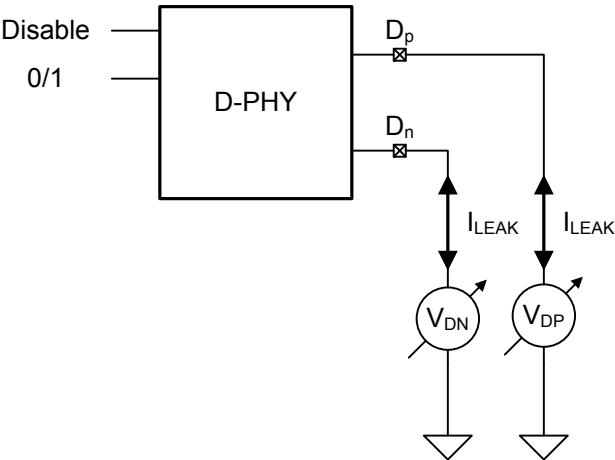
Figure 50 Pin Leakage Measurement Example Circuit
