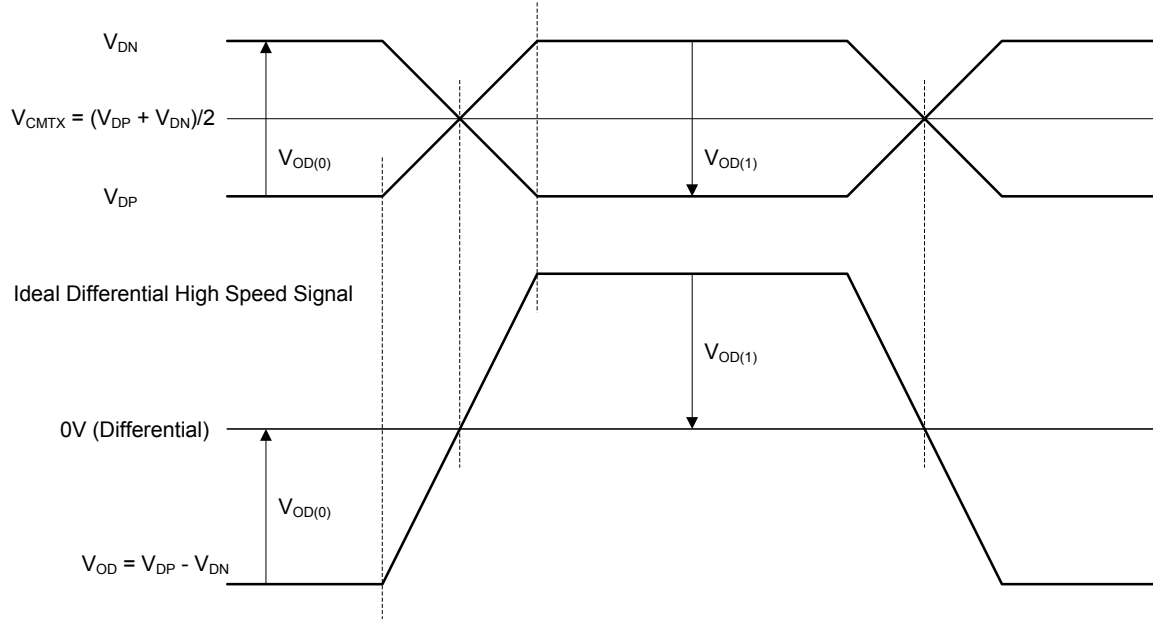
Figure 38 Ideal Single-ended and Resulting Differential HS Signals
