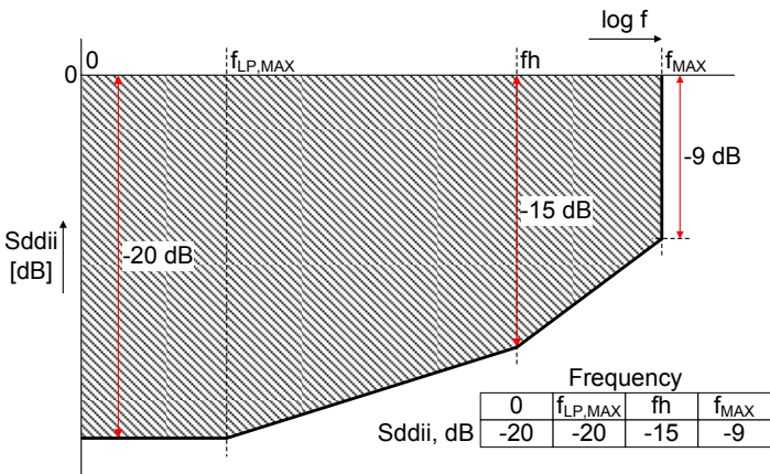
1236 1237 Figure 29 Template for Differential Reflection at Both Ports
